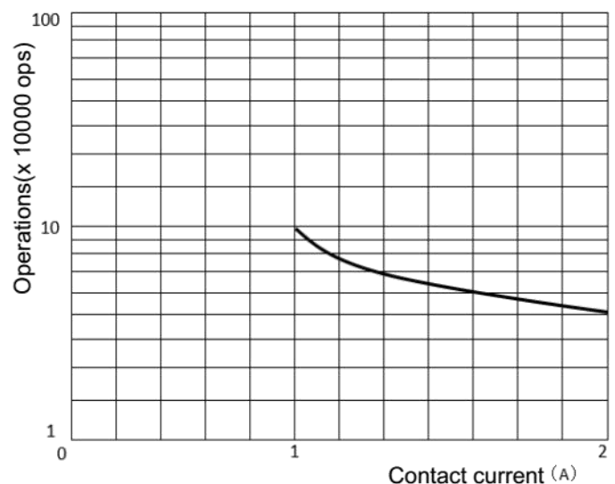
ENDURANCE CURVE
