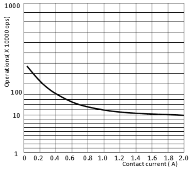
ENDURANCE CURVE
